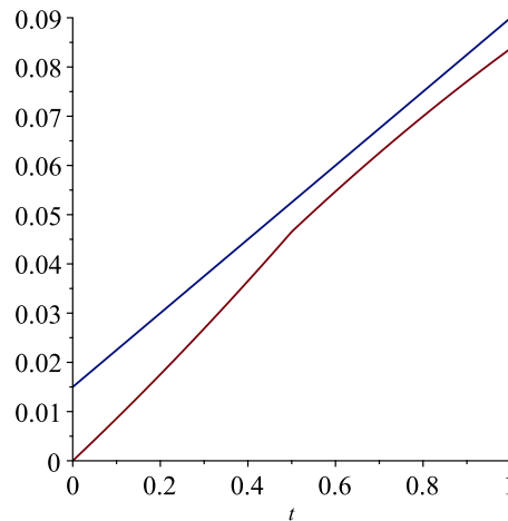
Fig. 1. \left| {}^C \mathcal{D}_{0+}^{\frac{3}{2}} y(t) + \sqrt{\pi} f(t, y(t)) \right| and \frac{1}{200} \varphi(t) = \frac{1}{200} (15t + 3) , t \in [0, 1] .
